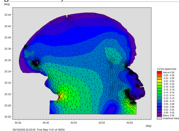
Figure 11. Changes in the current velocity of Chabahar Bay at a one-time step after calibration
