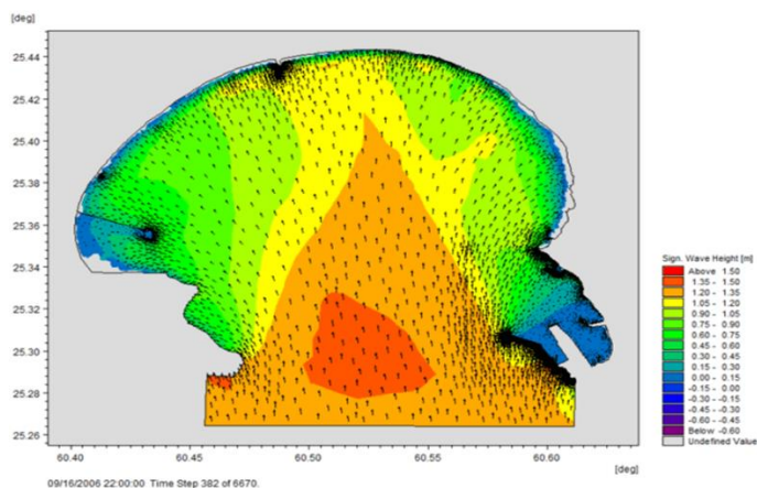
Figure 7. Wave height variations in Chabahar Bay for a one-time step after calibration
