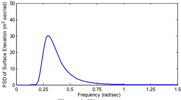
Figure 1. Wave spectrum
