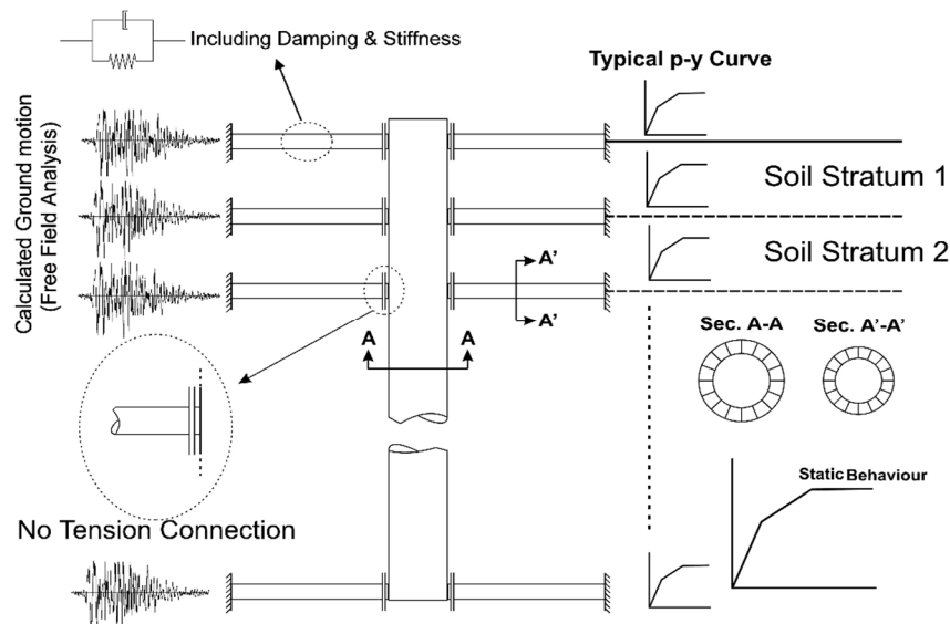
Figure 3. View of BNWF model for nonlinear dynamic response analysis of jacket pile using Fiber Elements
