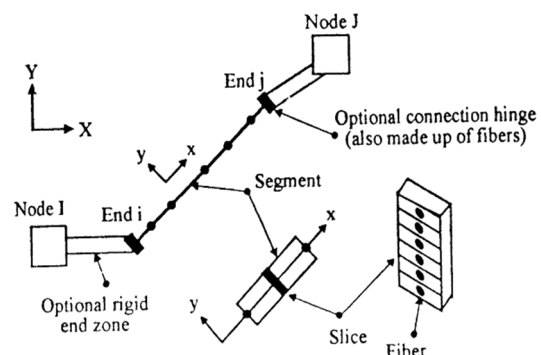
Figure 2. Element type 15 configuration [3], [20]
