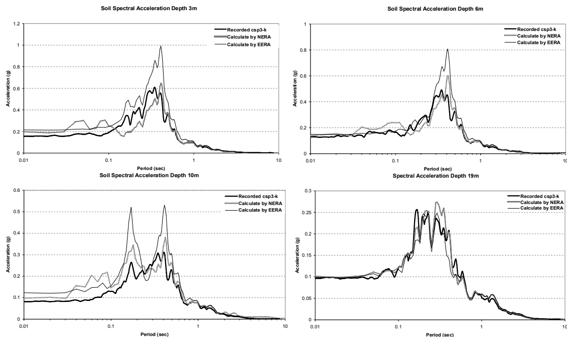
Figure 4. ARS of soil profile in CSP3-k
