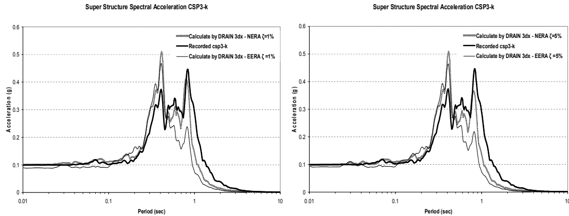
Figure 8. ARS of Superstructure CSP3-K
