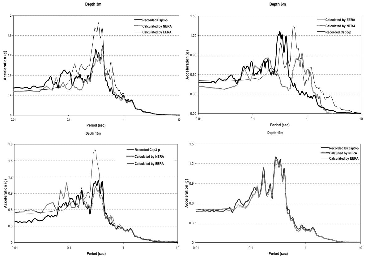
Figure 5. ARS of soil profile in CSP3-P
