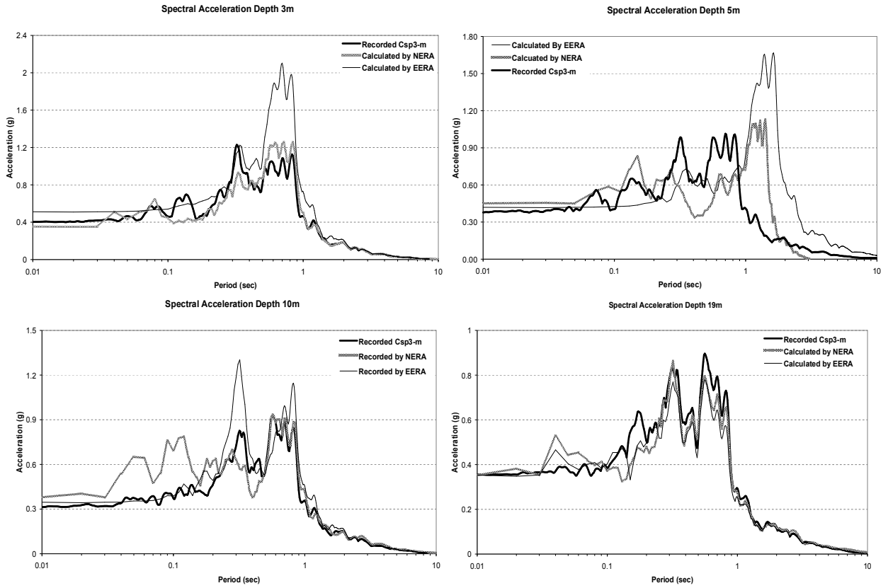
Figure 6. ARS of soil profile in CSP3-M
