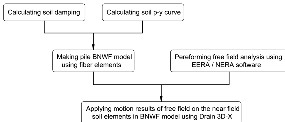
Figure 1. Steps for the nonlinear dynamic analysis of pile foundation subjected to strong ground motions
