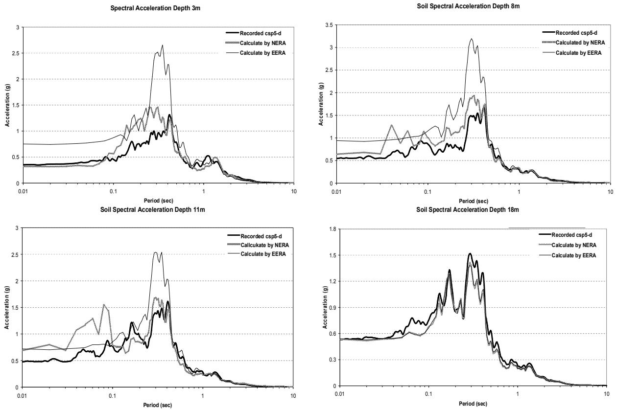
Figure 10. ARS of soil profile in CSP5-D
