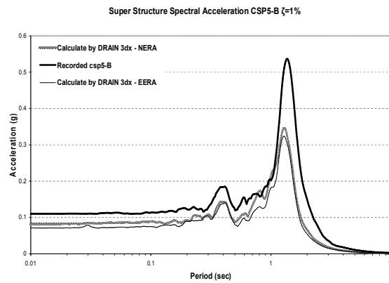
Figure 11. ARS of Superstructure in CSP5-B
