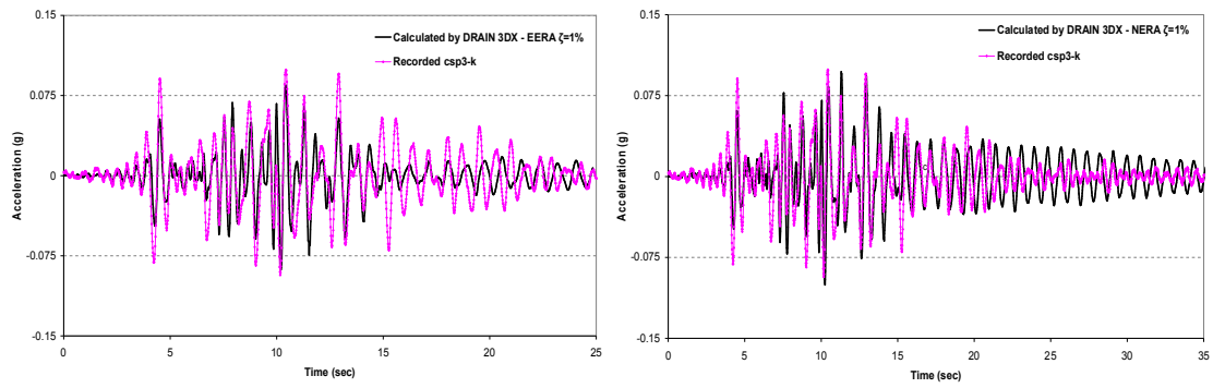
Figure 7. Super structure acceleration response CSP3-K ( \xi=1\% )
