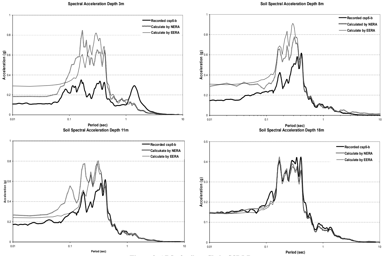
Figure 9. ARS of soil profile in CSP5-B
