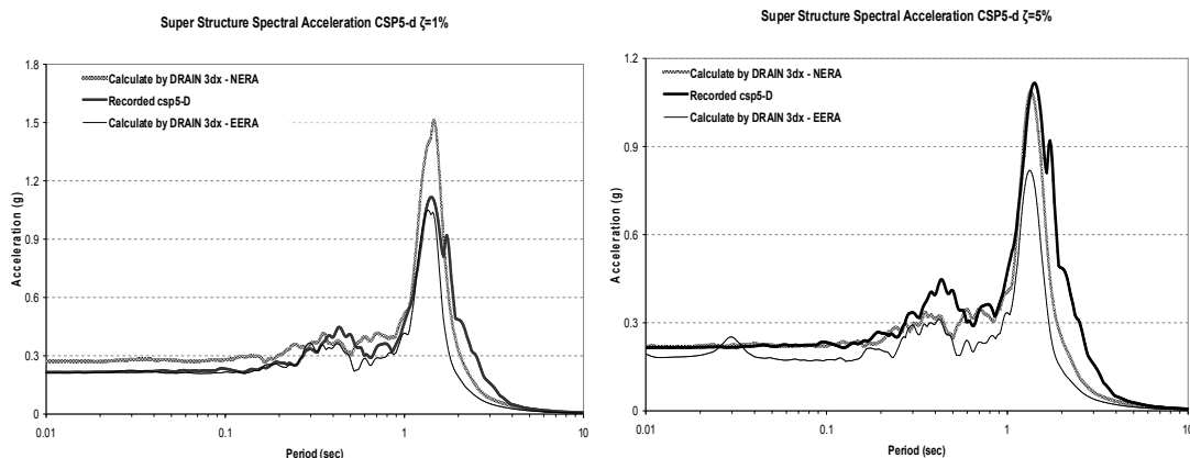
Figure 12. ARS of Superstructure in CSP5-D
