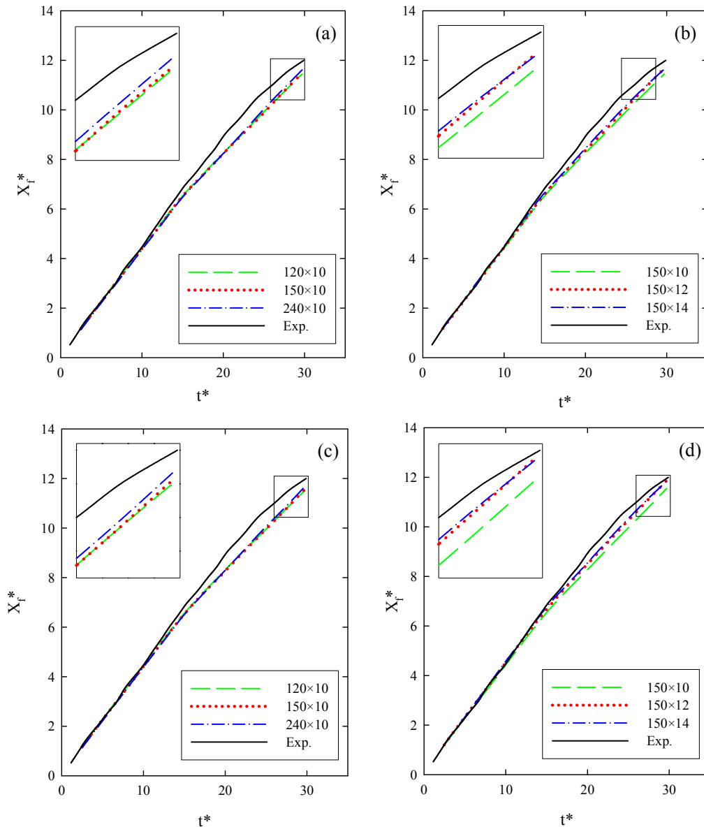
Figure 7. Simulated front position profiles for different grid resolutions with buoyant k-\varepsilon (a and b) and EARSM (c and d) turbulence closures in experiment of Zhu et al. [36]
