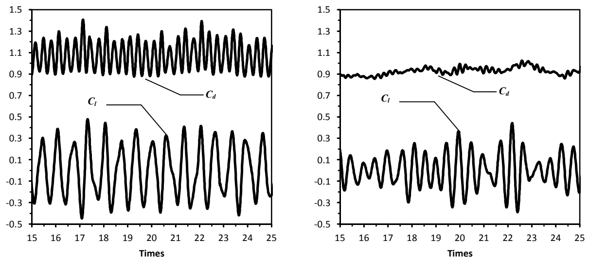
Figure 11. Drag ( C_d ) and lift ( C_l ) force coefficients time histories for the elastically mounted (left) and fixed (right) tapered circular cylinder at a reduced velocity of 6.47.
