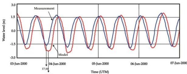
Figure 4: Comparing water level time series derived from the model (red) and recorded by the gauge at G1
