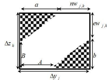
Figure 4. A mesh cell with porous walls;
