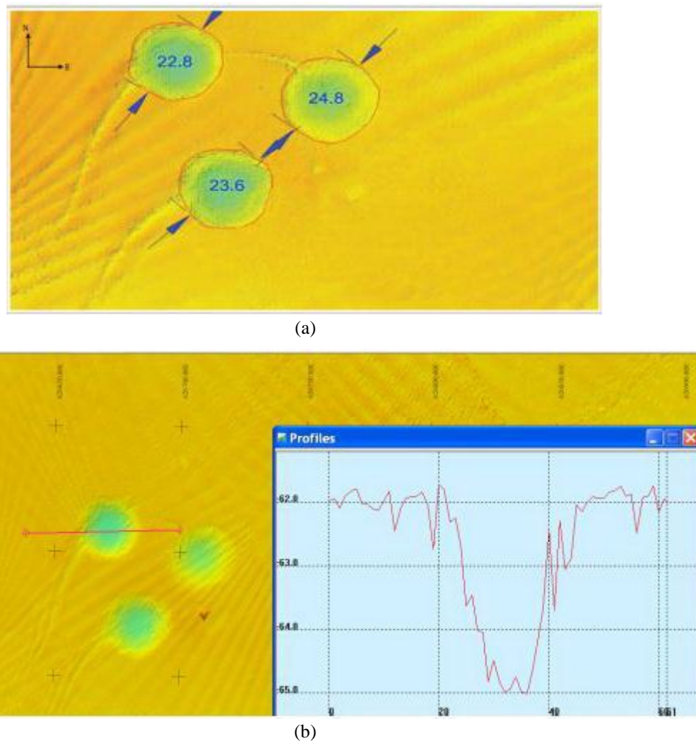
Figure 2. (a) Footprints in the seabed due to deployment of jack-up unit at the site of second case (b) Cross Profile on Footprint of Jack up Bow Leg for one leg (unit of axis is meter)
