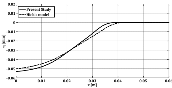
Figure 9. Comparison of elevated free surface profile for a circle with b = 0.5 and V_0 = 0.1 m/s with Hick's method.
