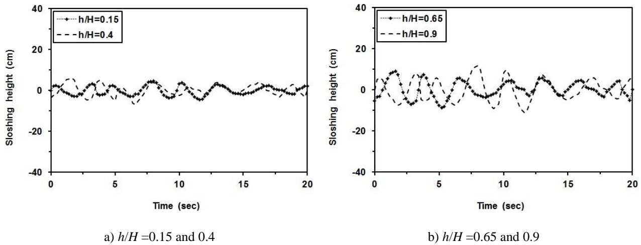
Fig. 13. Liquid sloshing height time histories for various baffle positions under the 1995 Kobe earthquake.
