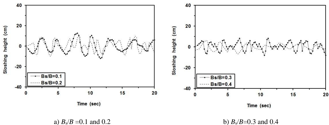
Fig. 14. Liquid sloshing time variations for various baffle widths.
