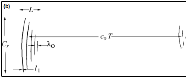
Figure 1. An example of internal waves by Landsat 8 on March 31, 2014 in the Persian Gulf (a); Schematic formation of internal waves on the fracture zone of the continental shelf (b) [2].
