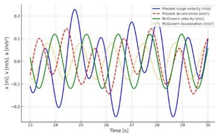
Figure 4. Validation of the maximum velocity and acceleration of the center of the floating plate surface
