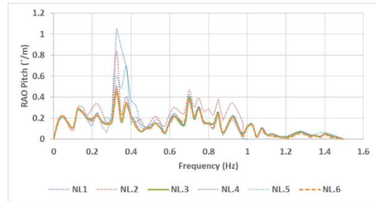
Figure 11. Comparing the results of model 6 with other nonlinear ones in pitch motion
