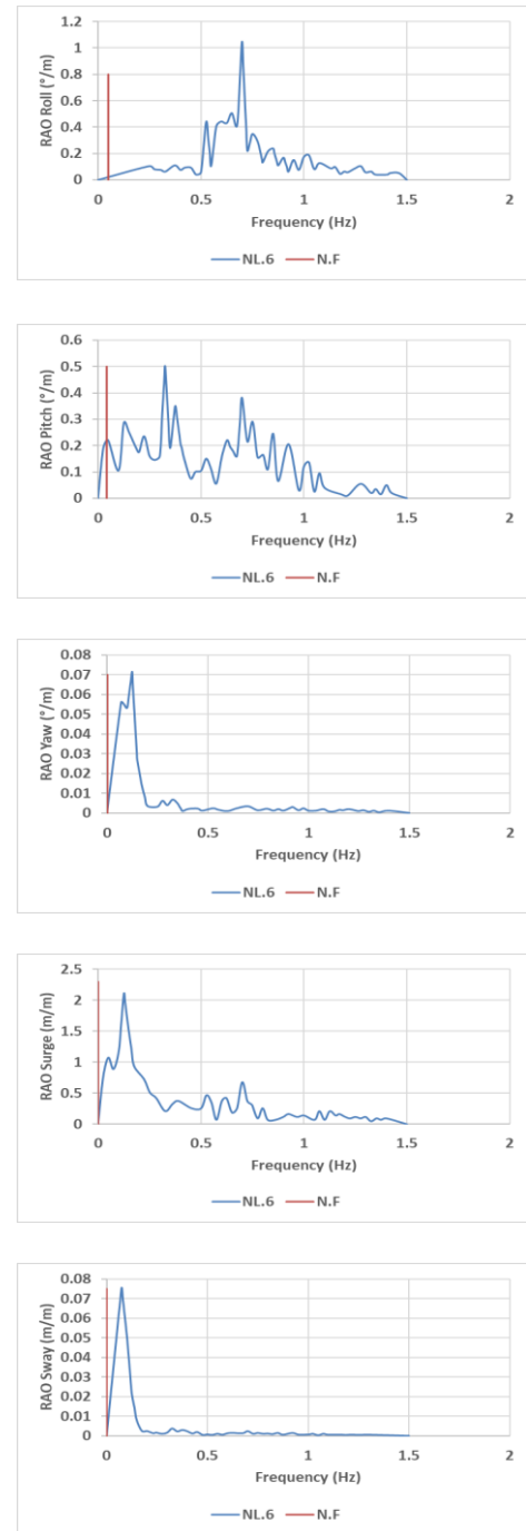
Figure 14. Position of natural frequency and dynamic motion frequency in finalized mode
