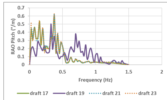
Figure 16. Comparative results of different draft depth in model 6
