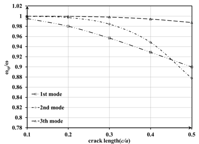
Figure 19. Effect of crack length on the natural frequency ratio of the simply-supported plate
