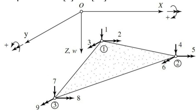
Figure 1. A triangular shell element
