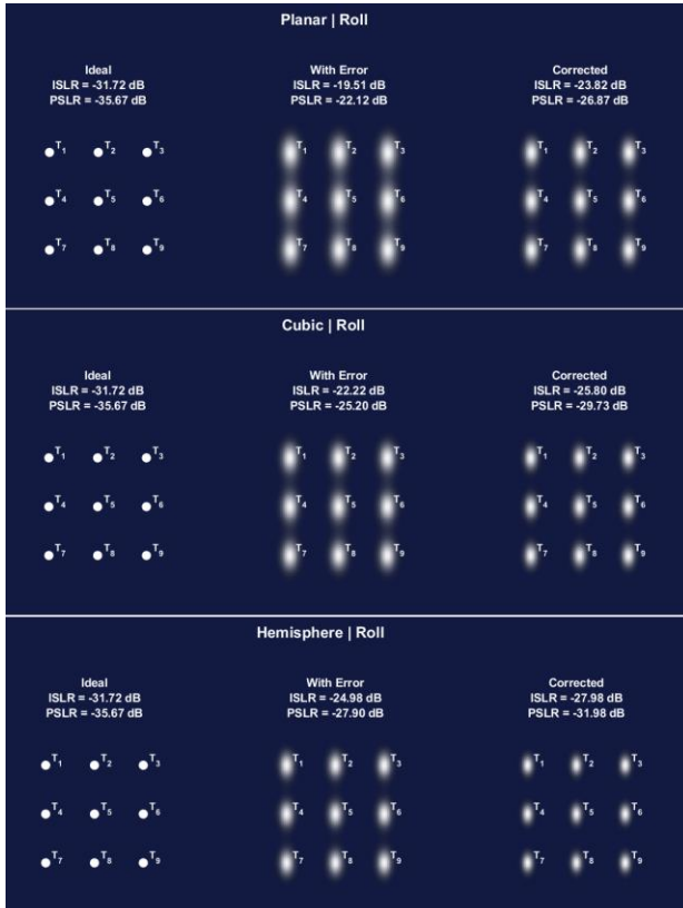
Figure 10. Roll motion: mean PSLR/ISLR for planar, cubic, and hemispherical arrays (Ideal, With Error, Corrected)
