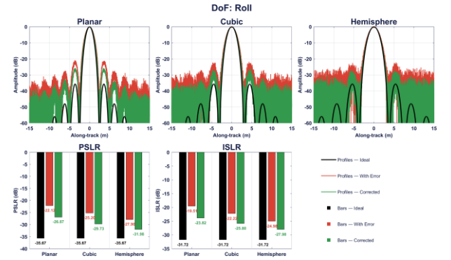
Figure 9. Mean over Roll: PSLR and ISLR Comparison Among Planar, Cubic, and Hemispherical Arrays
