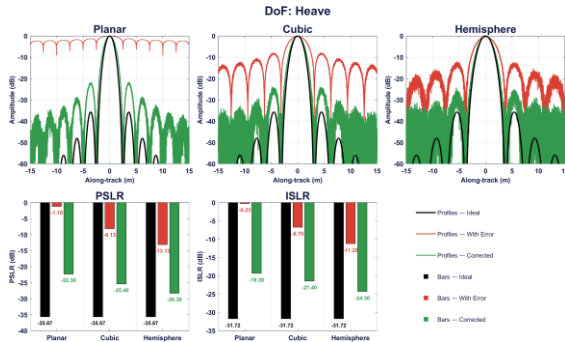
Figure 8. Mean over Heave: PSLR and ISLR Comparison Among Planar, Cubic, and Hemispherical Arrays
