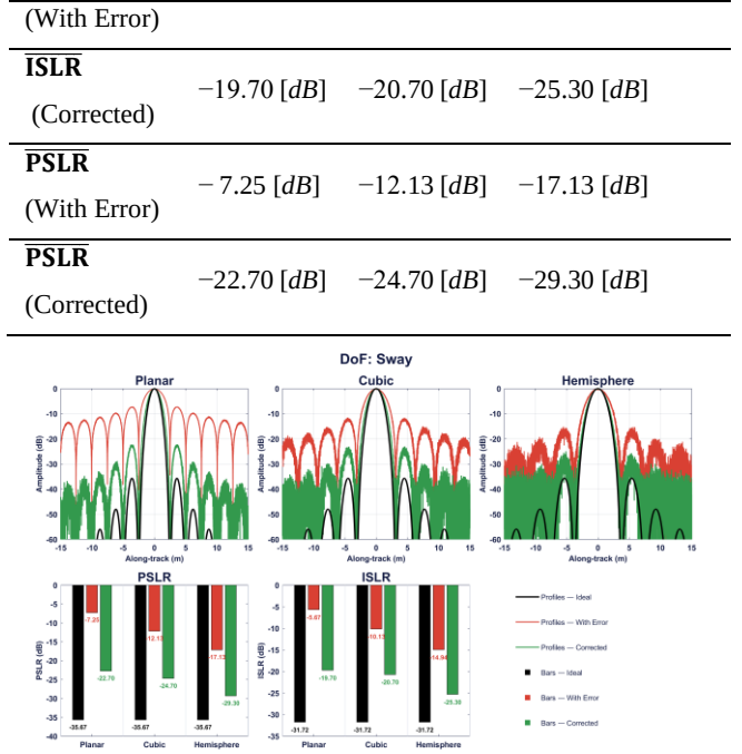
Figure 7. Mean over Sway: PSLR and ISLR Comparison Among Planar, Cubic, and Hemispherical Arrays
