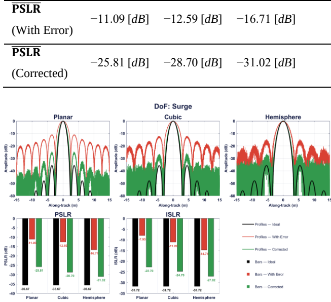
Figure 5. Mean over Surge: PSLR and ISLR Comparison Among Planar, Cubic, and Hemispherical Arrays
