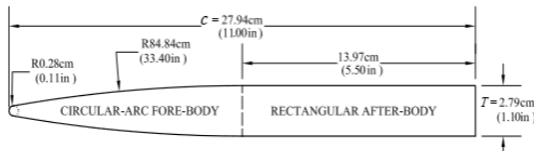
Fig. 4: A view of the Casey Harwood's foil [28]
