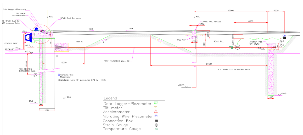
Figure 2. Cross-section of SHM drawing of harbour structure of Shahid Rajaei port (phase 3) development
