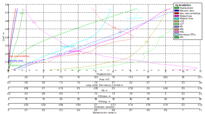
Figure 23. Curves illustrating variations in important hydrostatic parameters at various waterlines with a trim of 1.0 meter towards the float heel.
