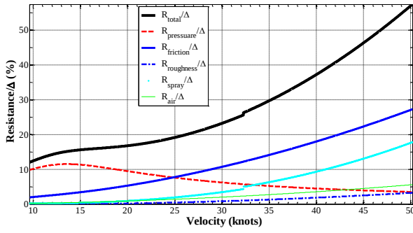
Figure 37: Ratio of resistance components to vessel weight at the initial trim angle of 5.1 degrees and LCG=2.441 m.
