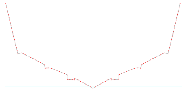
Figure 14. Display of section 4000 as an example (Red dots on the section indicate the offset replacement points)
