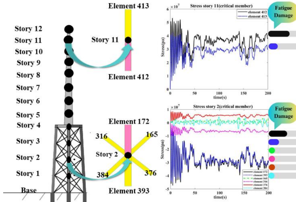
Figure 2. finding critical members of the structure after dynamic analysis
