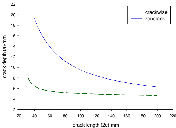
Figure10. Comparison of BS7910 guideline and FE method at \epsilon = 0.3\%
