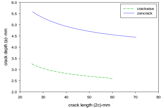
Figure12. Comparison of BS7910 guideline and FE method at \epsilon = 1.2\%
