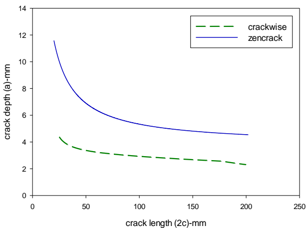
Figure11. Comparison of BS7910 guideline and FE method at \epsilon = 0.8\%
