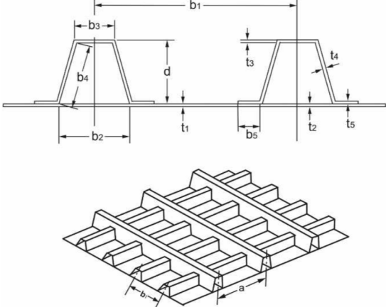
Figure 2. Geometrical details of the stiffened plates in deck, side shell and bilge of the composite ship [9].
