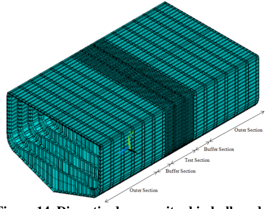
Figure 14. Discretised composite ship hull model.
