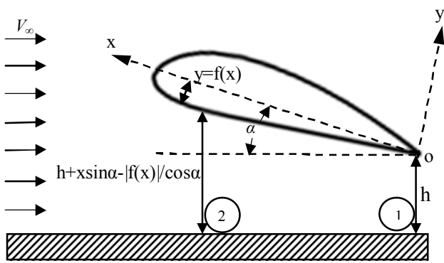
Figure 1, Schematic diagram for the mathematical model of airfoil in ground effect
