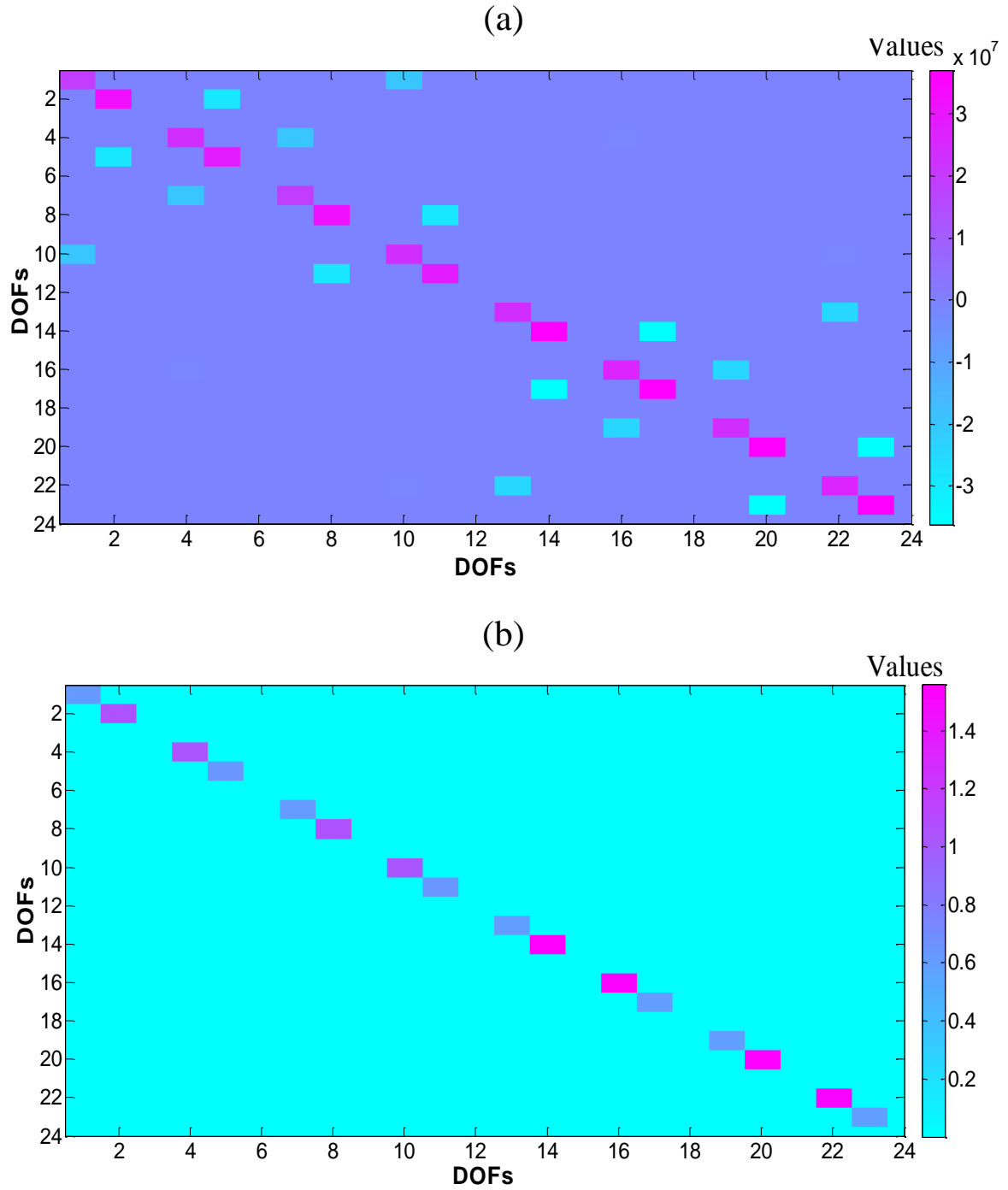
Figure 3. (a) Initial stiffness matrix (b) Initial mass matrix of platform model
