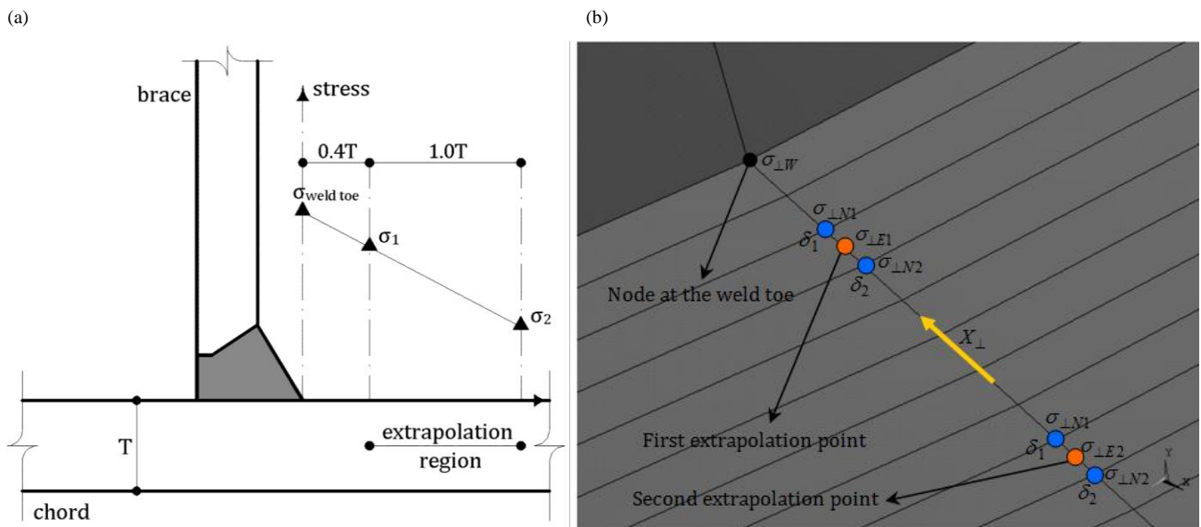
Figure 4. (a) Extrapolation procedure recommended by IIW-XV-E [51], (b) Required interpolations and extrapolations to extract SCFs based on the stresses perpendicular to the weld toe
