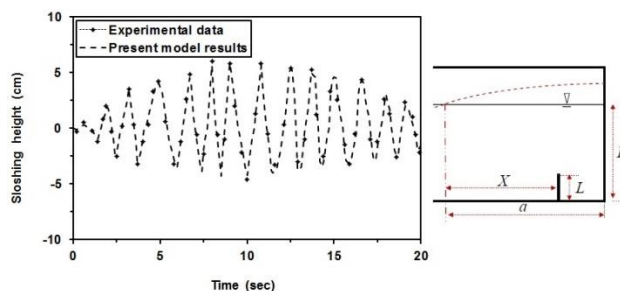
Fig. 4. Comparison of the wave height with the experimental results of Goudarzi and Sabbagh-Yazdi [29].
