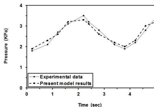
Fig. 5. Comparison of the pressure with the experimental results of Akyildiz and Unal [31].
