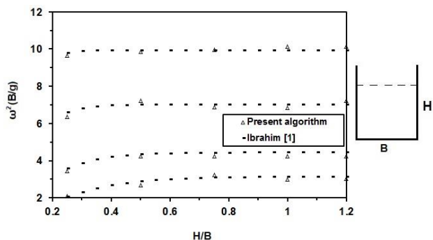
Fig. 2. Dimensionless sloshing frequencies for various liquid depths.
