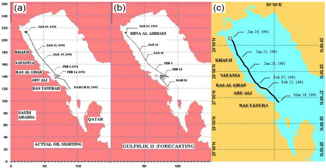
Figure 2. Comparison between real oil spill trajectory (a) [29], oil spill trajectory simulated by GULFSLIK model (b) [29], oil spill trajectory simulated by OSCAR model (c) [Ranjbar et al.] during January 19, 1991, to March 18, 1991
