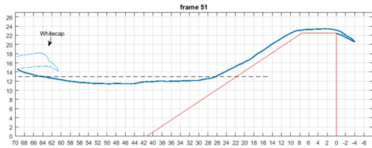
Figure 7. Wave run-up on slope 1:1.5, SWL 13 cm, T=0.75 sec, H=6 cm. Time step between successive frames is 0.05 sec
