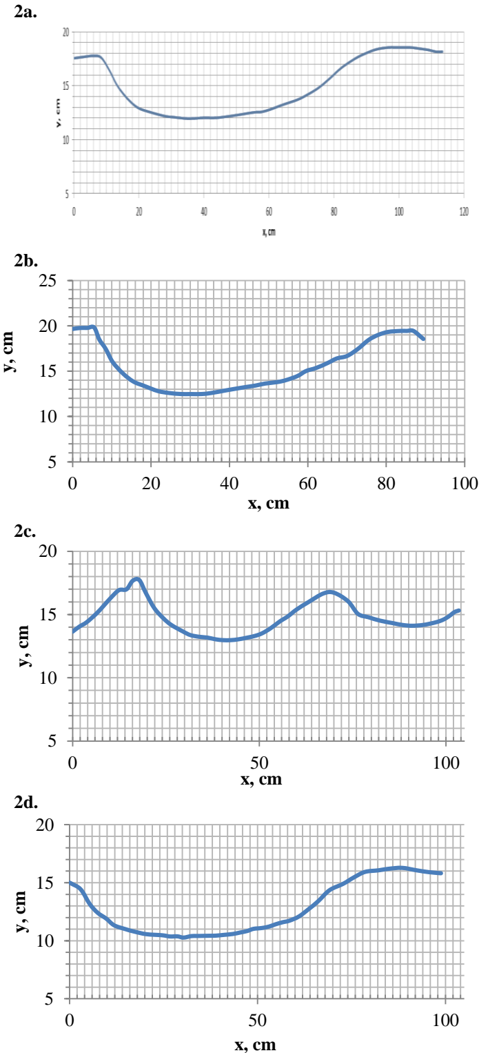
Figure 2. Input waves; water surface from high-speed images has been captured using web-based image processing software [12]
