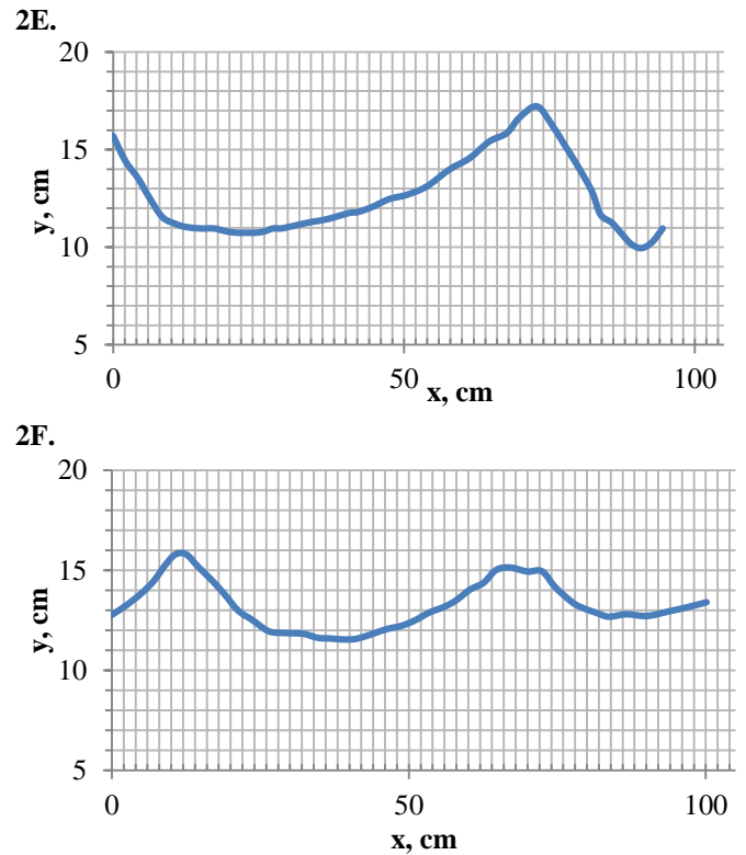
Figure 2. Input waves; water surface from high-speed images has been captured using web-based image processing software [12]
