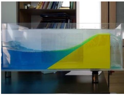
Figure 7. Wave run-up on slope 1:1.5, SWL 13 cm, T=0.75 sec, H=6 cm. Time step between successive frames is 0.05 sec
