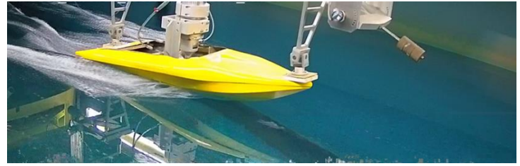
Fig. 7. Model Testing Without Trim Tabs at 2 m/s
